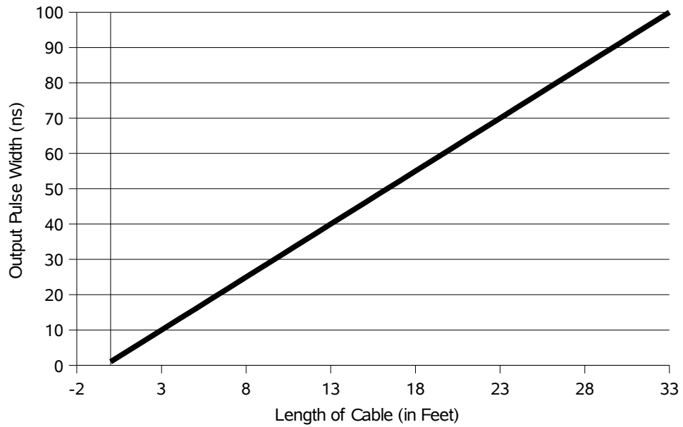
Pulse Width / Cable Length Relationship
